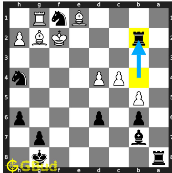
Figure 4: Rb2+
